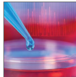
Flow Cytometry
