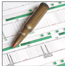
Capillary Electrophoresis
