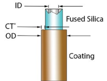
Polymicro Technologies™ Polymide Capillary Tubing
