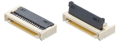
0.50mm Pitch FFC/FPC Connector, FBH2 Series, Easy-On Actuator, Back Flip Dual-Contact
