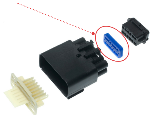
Exploded View of an MX150 Plug with Matte Seal (Blue), Which Eliminates the Need and Cost for Individual Wire Seals
